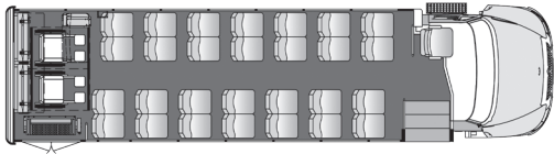
28 Passenger 2 Wheelchair with Flip and Foldaway Seats Plus Driver
